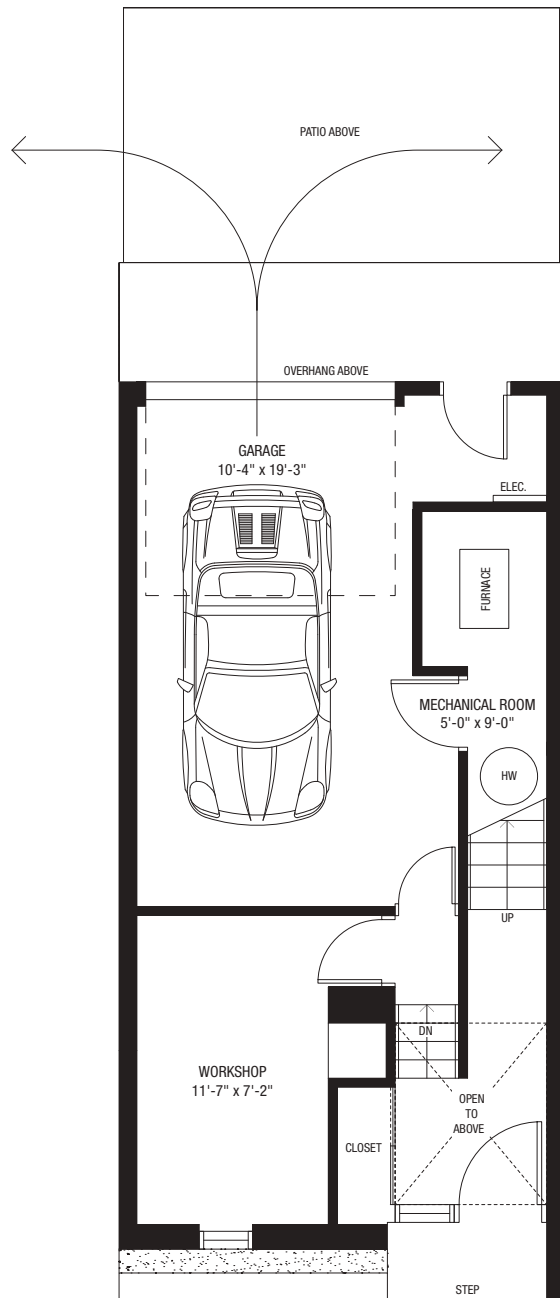
BASEMENT
