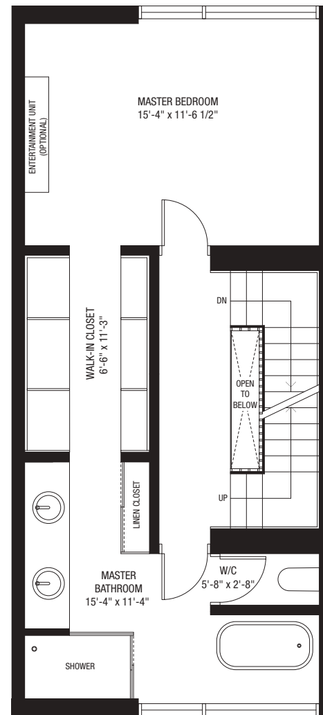
SECOND FLOOR
