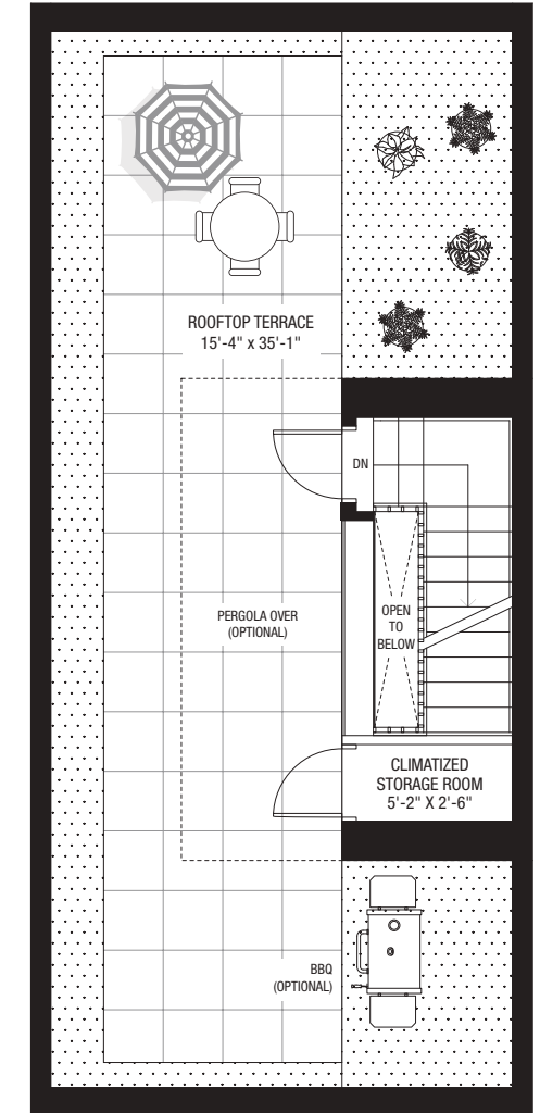
ROOFTOP TERRACE
